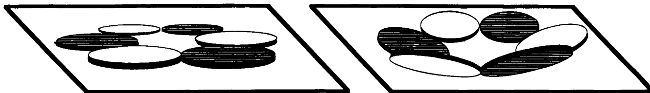
Figure 9. Differences in the planarity of the rosette of an aggregate (as calculated using molecular dynamics) can be correlated with the stability of that aggregate. An aggregate observed to have a rosette with an average structure close to planar (left) is more stable than one in which the rosette is nonplanar or fluctuates from planarity (right).
