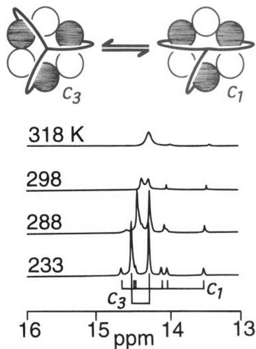
Figure 7. Low-temperature ^1\text{H} NMR spectroscopy resolves two conformational isomers—one having C_3 symmetry and the one having C_1 symmetry—of \text{hub}(\text{M})_3\text{:}3\text{barbital} . The two isomers are represented at the top of the figure (as viewed from above). The resonances between 13 and 16 ppm are the imide resonances that are identified with numbers. The C_3 isomer has two nonequivalent imide 31 resonances of barbital while the C_1 isomer has six nonequivalent resonances.
