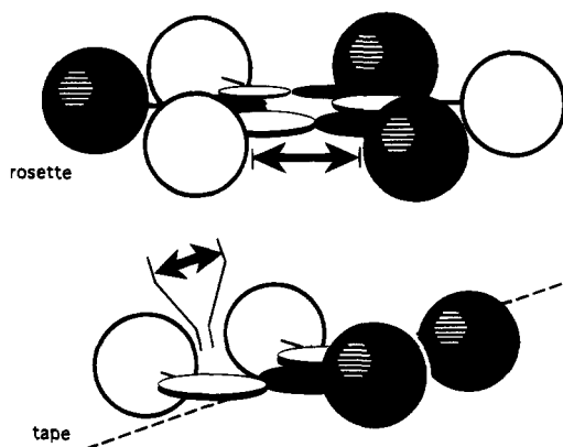
Figure 2. Preorganization describes the connection of melamines (or isocyanurates) using covalent bonds in a way that minimizes the unfavorable entropy of forming an aggregate. Peripheral crowding describes the use of bulky groups that favor rosette motifs over tape motifs. The arrows indicate regions of potential steric overlap.
