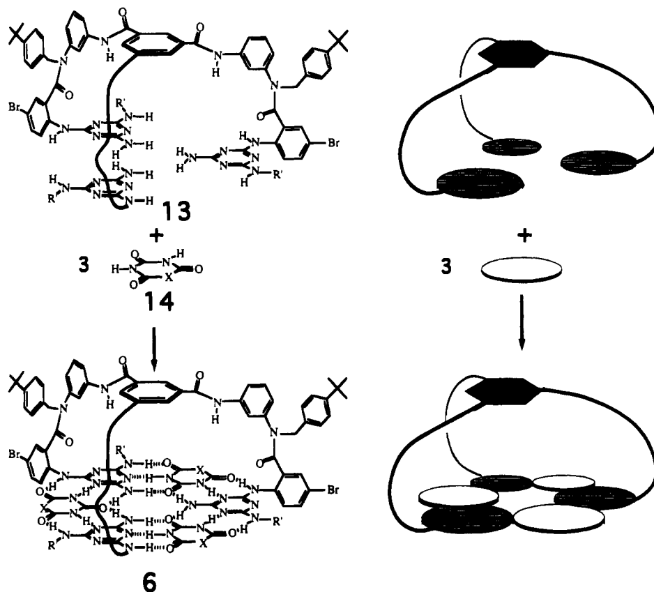
Figure 4. \text{hub}(\text{M})_3 (13). \text{R}' = (\text{CH}_2)_2\text{C}(\text{CH}_3)_3 . \text{X} = \text{NR}' (neo-hexylisocyanuric acid, 14).
