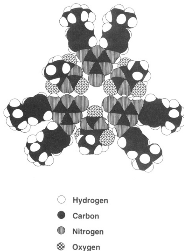
Figure 8. Crystal structure of the rosette composed of barbitalic acid and bis( p - tert -butylphenyl)melamine.
